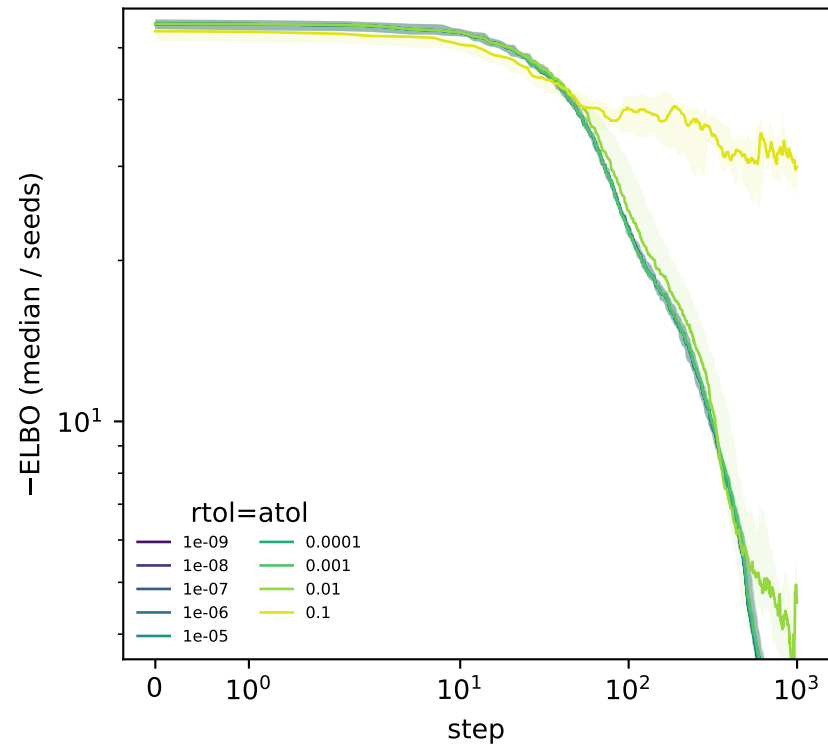
K=50 hier. mixture, dopri5 tol sweep
