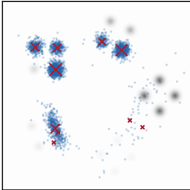
\eta_0 = 0.01 n_{eff}=7/50
