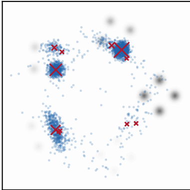
\eta_0 = 0.005 n_{eff}=6/50
