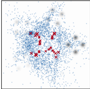
\eta_0 = 0.001 n_{eff}=33/50
