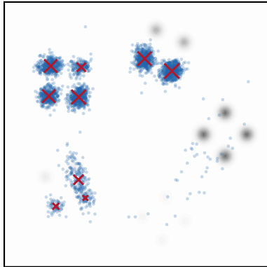
\eta_0 = 0.02 n_{eff}=8/50
