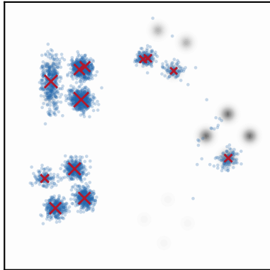
\eta_0 = 0.05 n_{eff}=11/50
