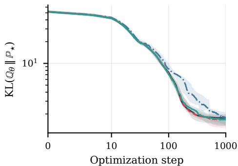
Hierarchical mixture, K=50
