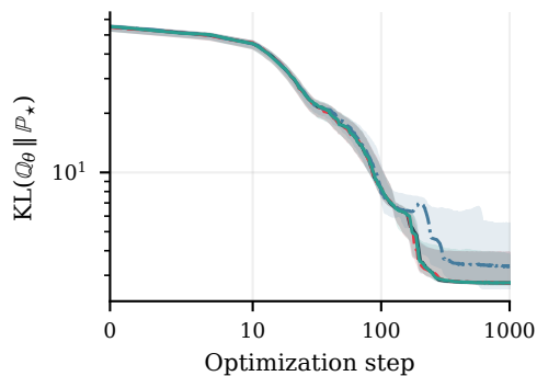
Hierarchical mixture, K=5
