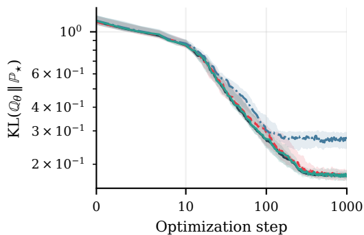
Hierarchical mixture, K=50
