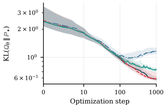
Hierarchical mixture, K=5
