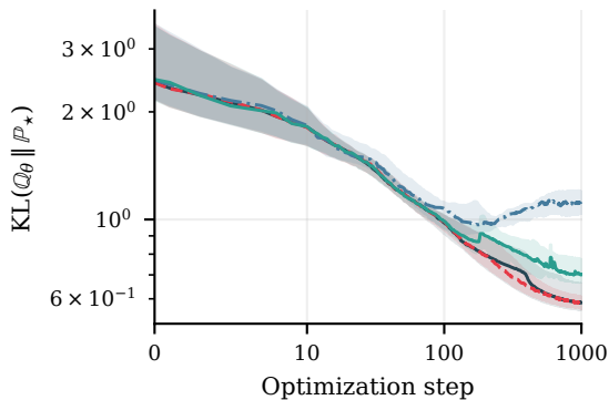
Rosenbrock, n=10
