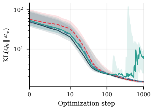
Rosenbrock, n=20
