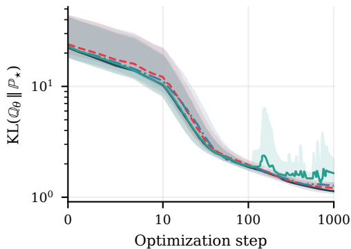
Rosenbrock, n=10
