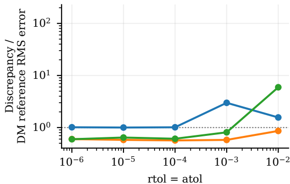
Hierarchical mixture, K=5 — DOPRI5
