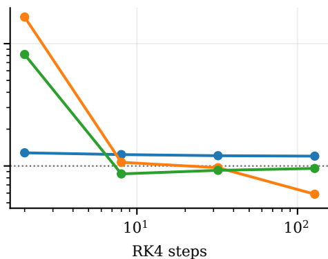
Rosenbrock — RK4
