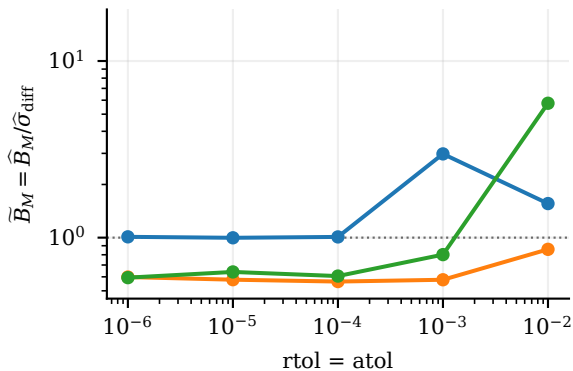
Hierarchical mixture, K=5 — DOPRI5
