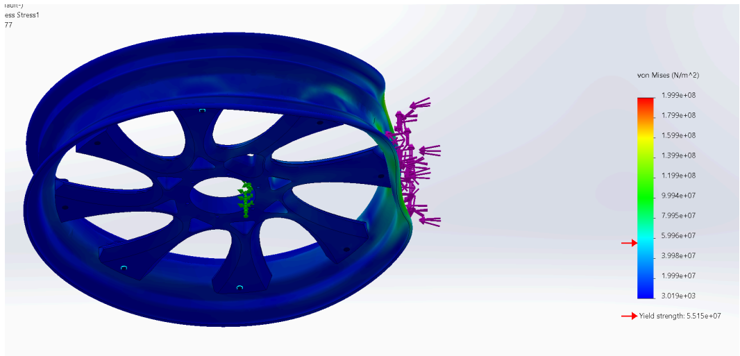
FEA Simulation Results
