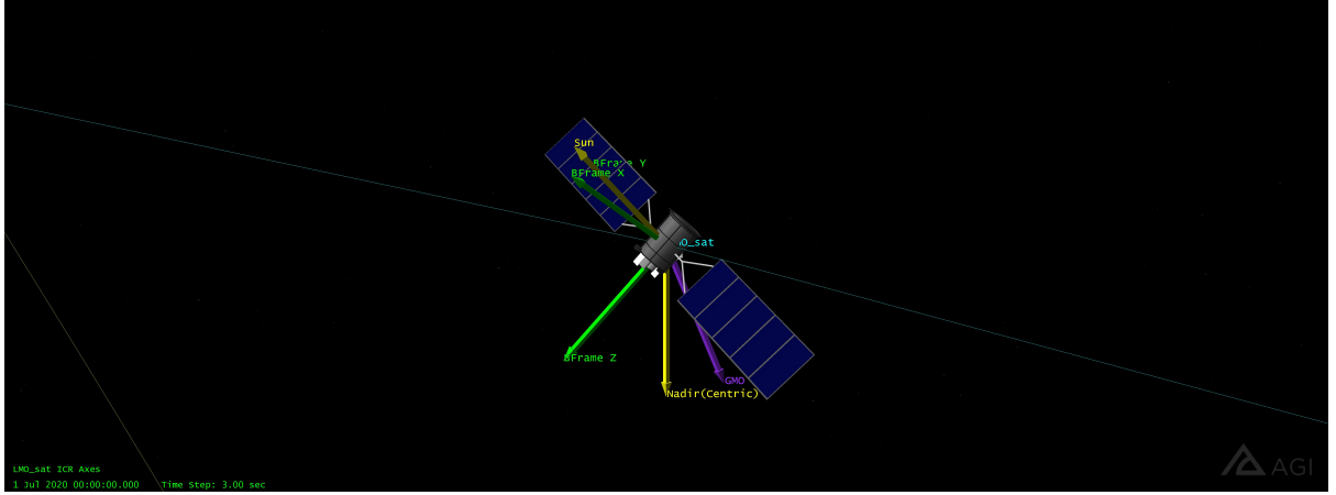
Figure 4.2: LMO spacecraft inertial state, body frame axes and Sun-, Nadir- and GMO-pointing vectors
