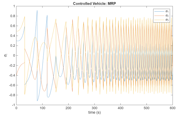
(f) \mathbf{u}_2 Applied: \sigma_{B/N}
