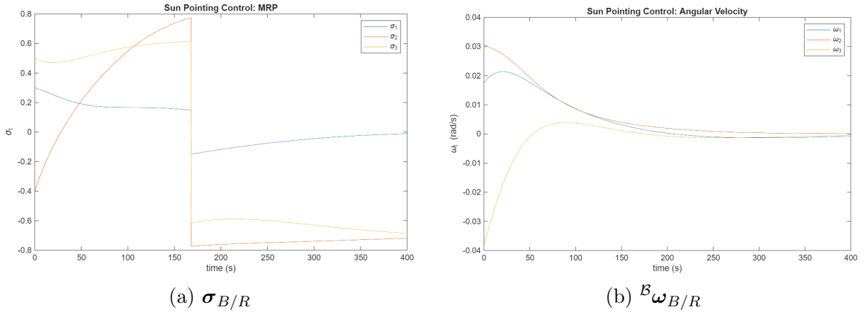
Figure 3.2: Results of Sun pointing control
