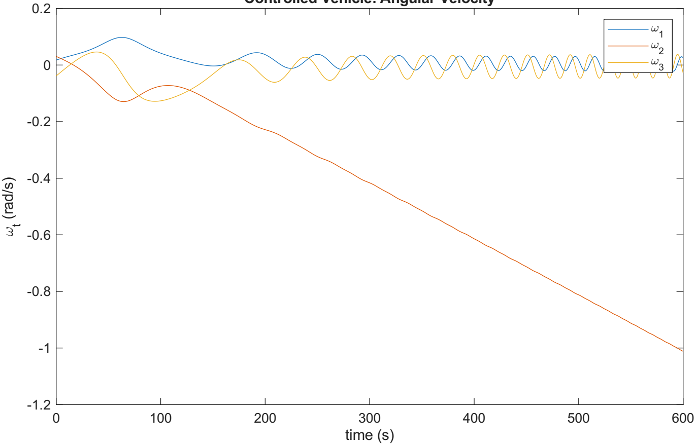
Controlled Vehicle: Angular Velocity
