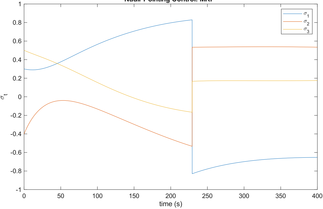
Nadir Pointing Control: MRP
