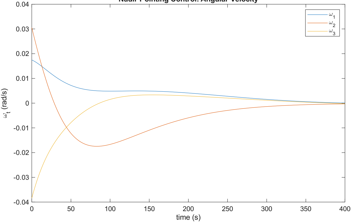
Nadir Pointing Control: Angular Velocity
