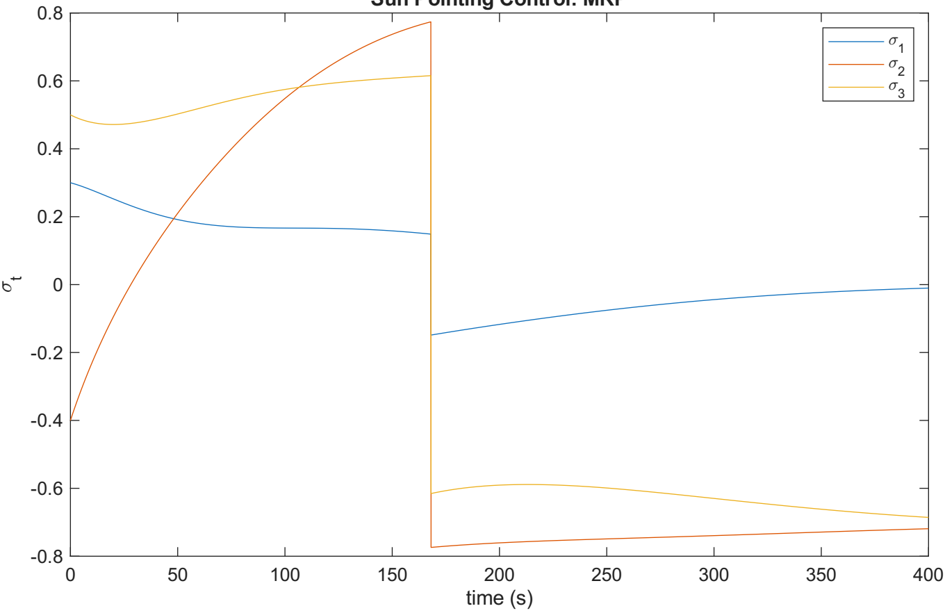
Sun Pointing Control: MRP
