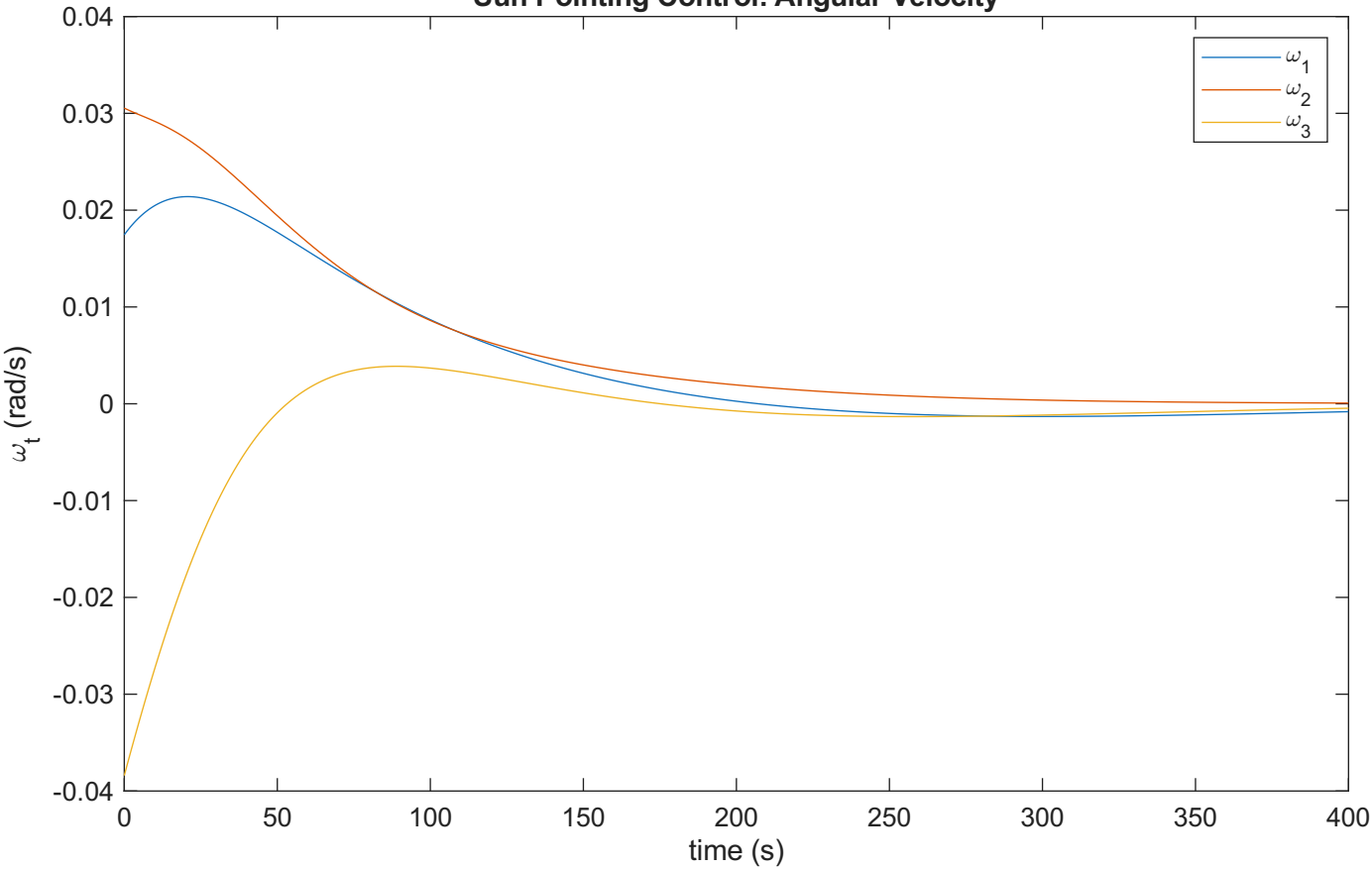
Sun Pointing Control: Angular Velocity
