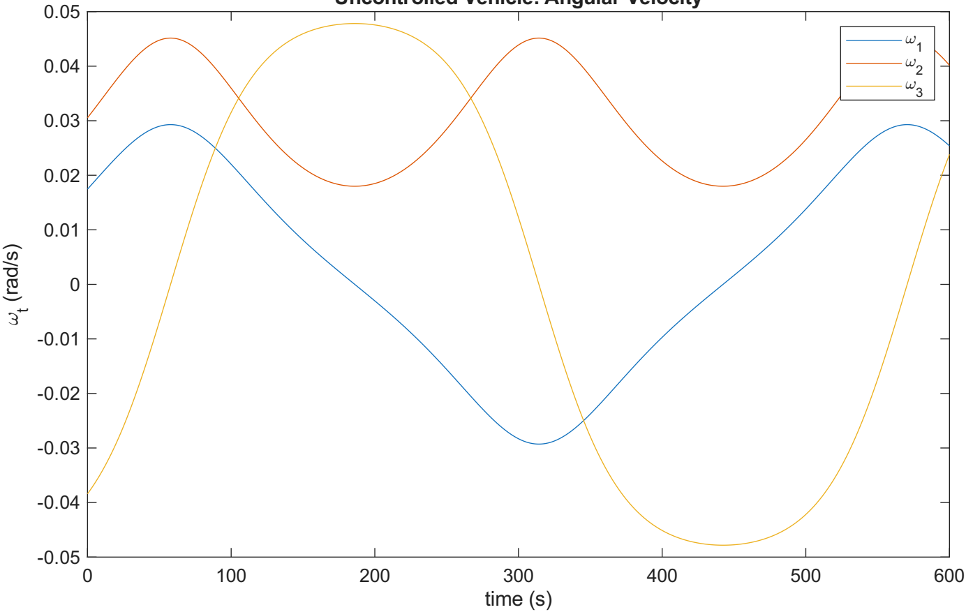
Uncontrolled Vehicle: Angular Velocity
