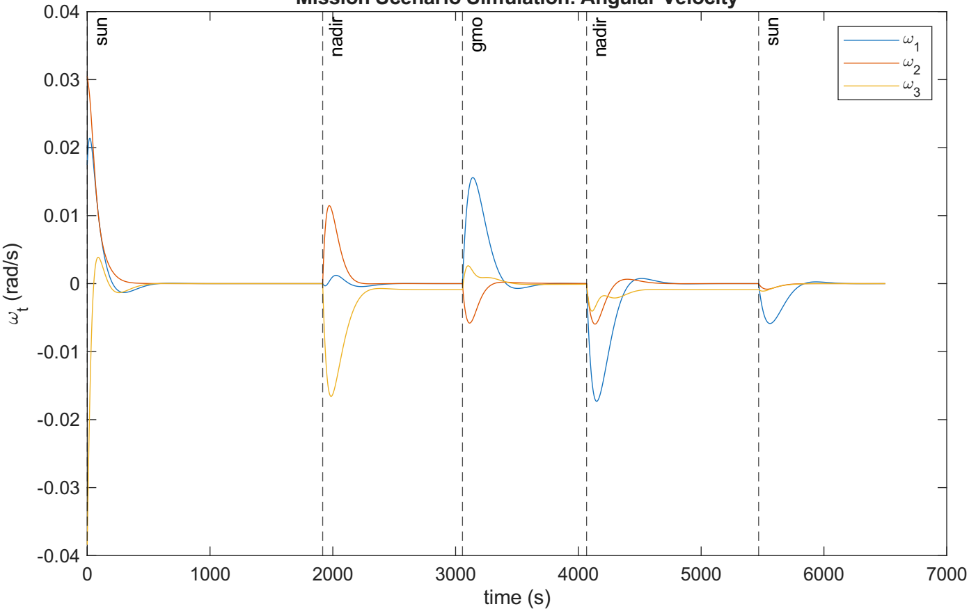
Mission Scenario Simulation: Angular Velocity
