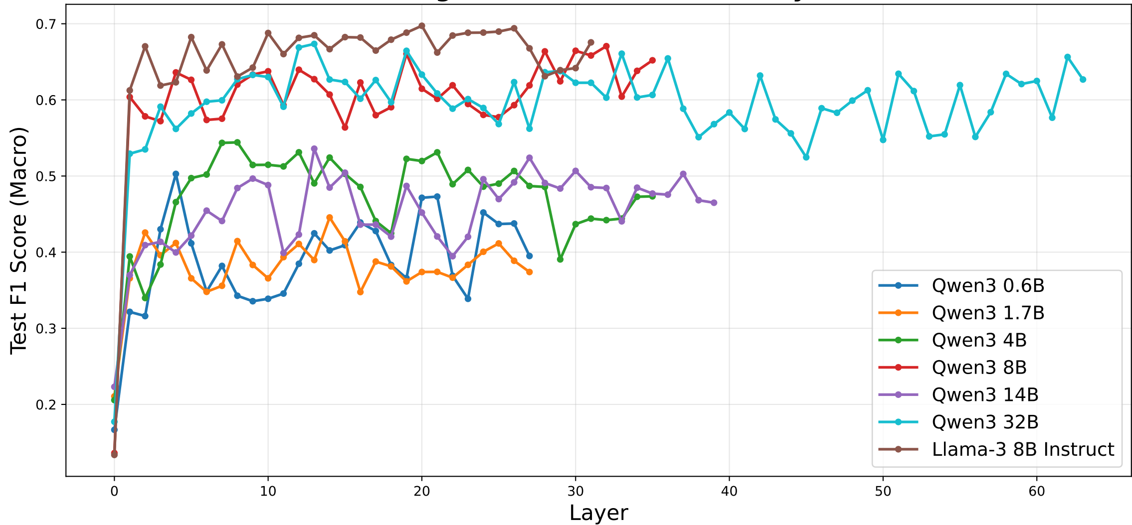
Probing Test F1 Scores Across Layers
