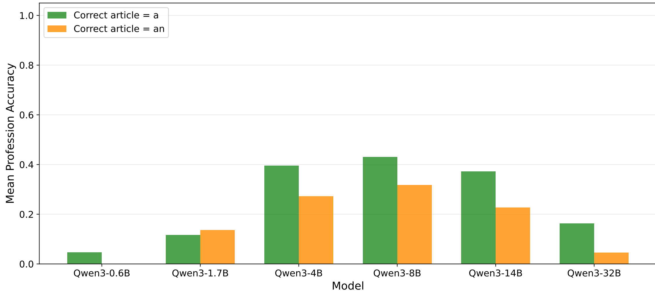
Mean Profession Accuracy by Correct Article Given Incorrect Article
