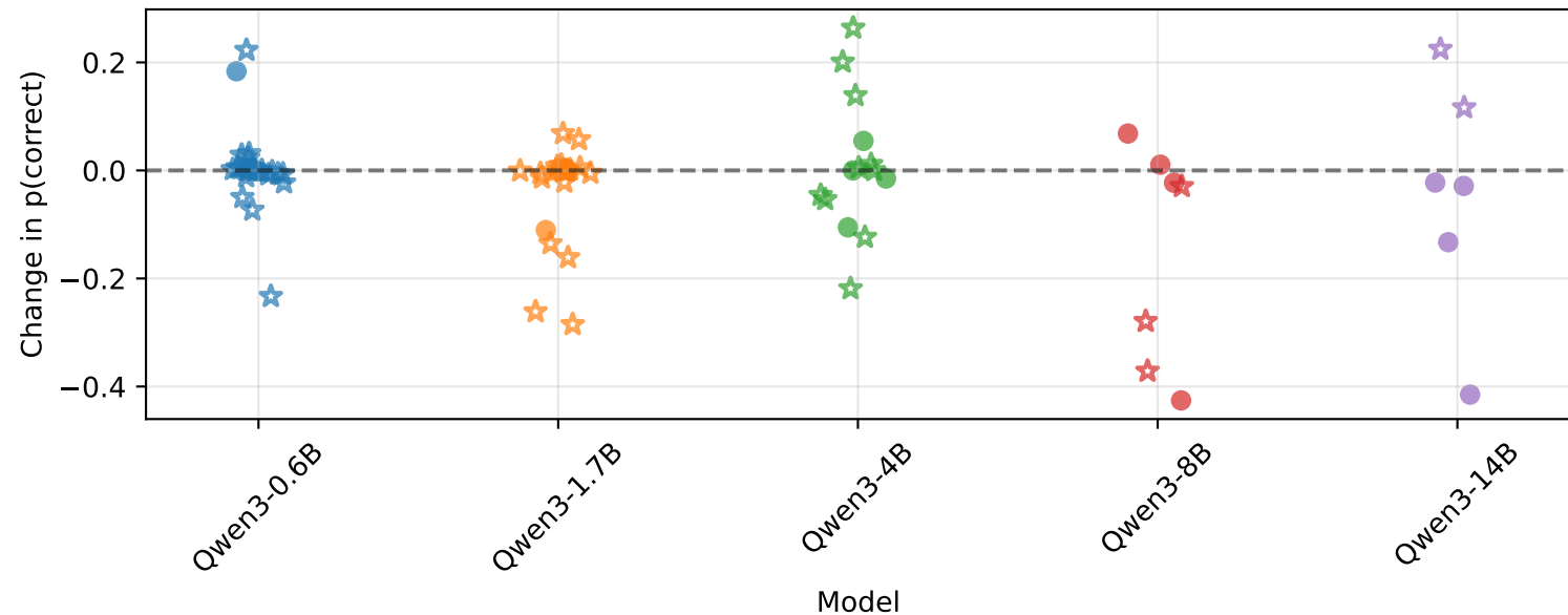
Effect of Multiplying Interventions on p(correct)
