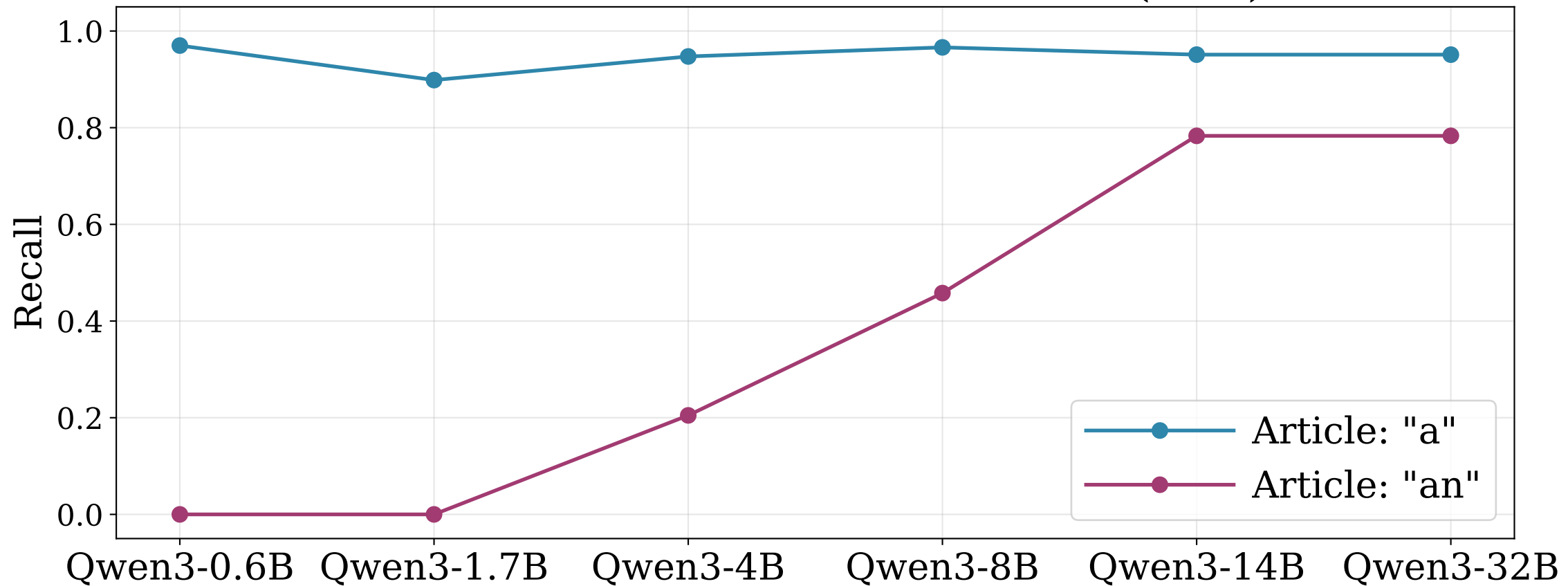
Article Recall Across Model Sizes (a/an)
