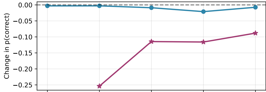
Direct Multiplying Interventions on p(correct)
