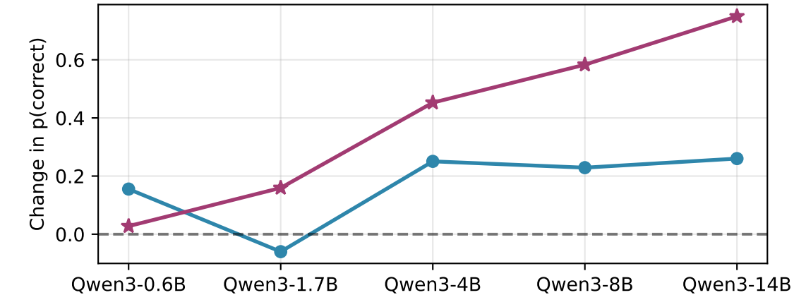
Multiplying Interventions on p(correct)
