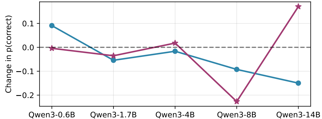
Direct Multiplying Interventions on p(correct)
