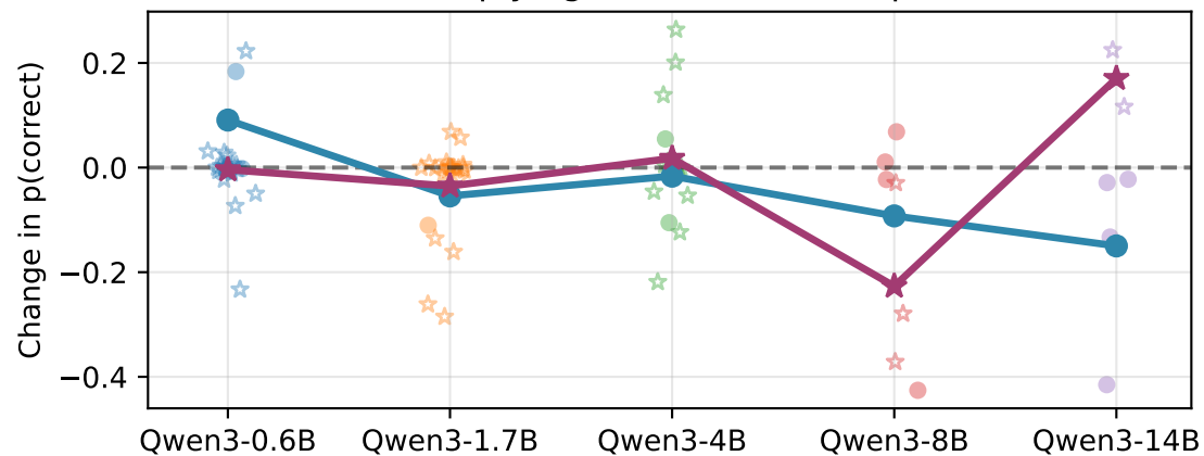
Direct Multiplying Interventions on p(correct)
