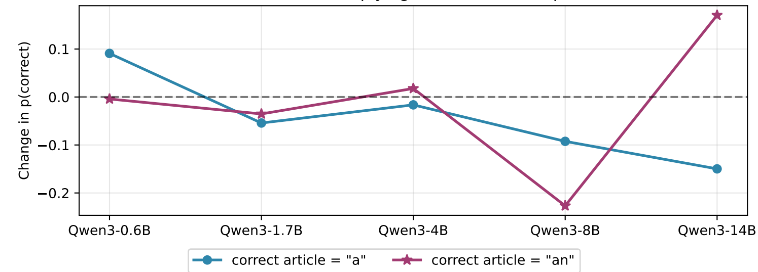
Effect of Direct Multiplying Interventions on p(correct)
