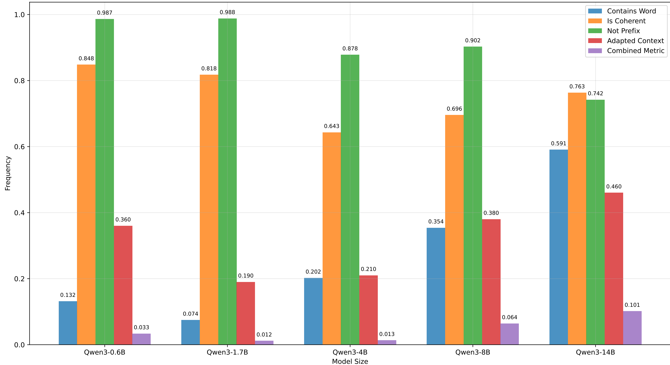
Model Steering Metrics by Size
