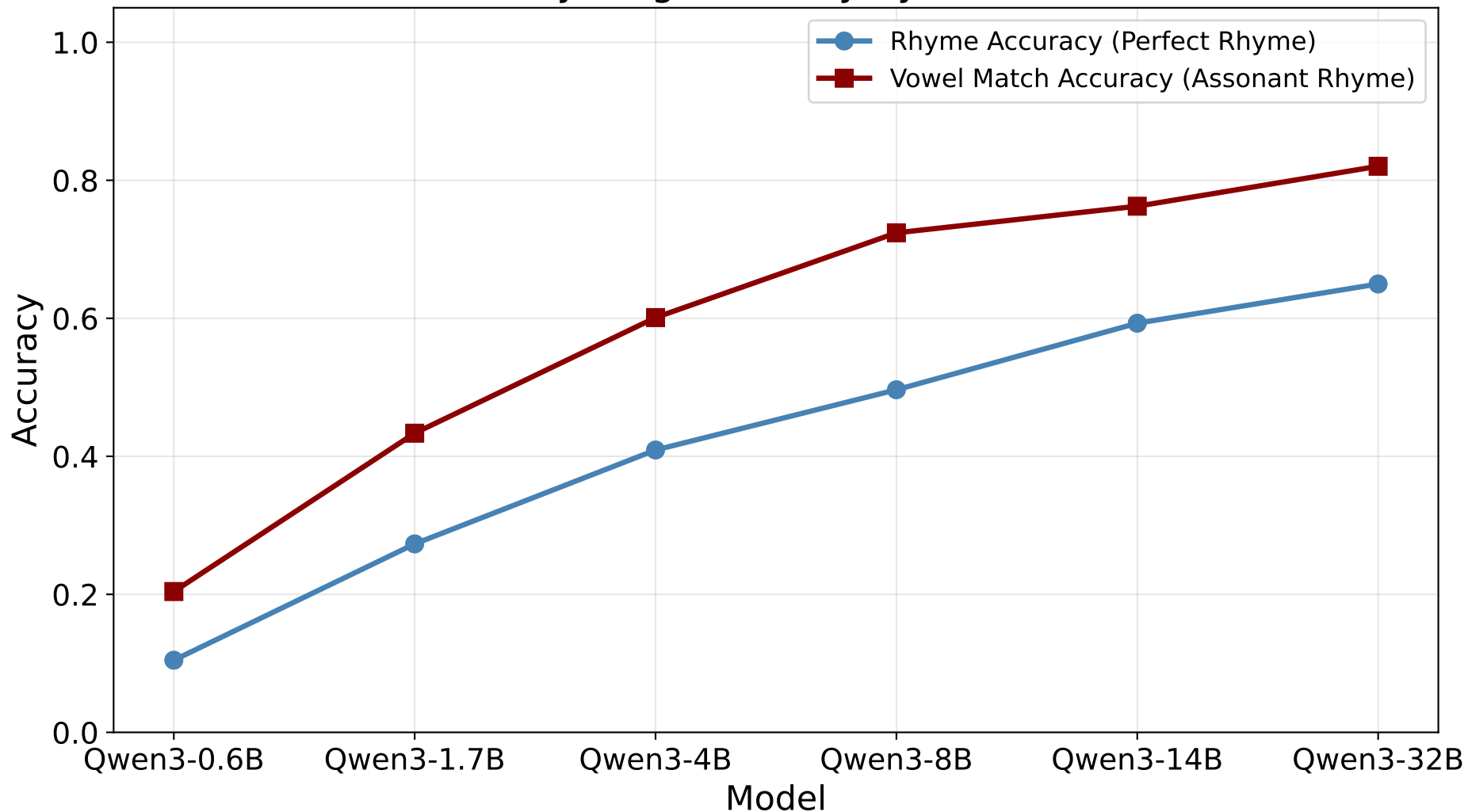
Rhyming Accuracy by Model
