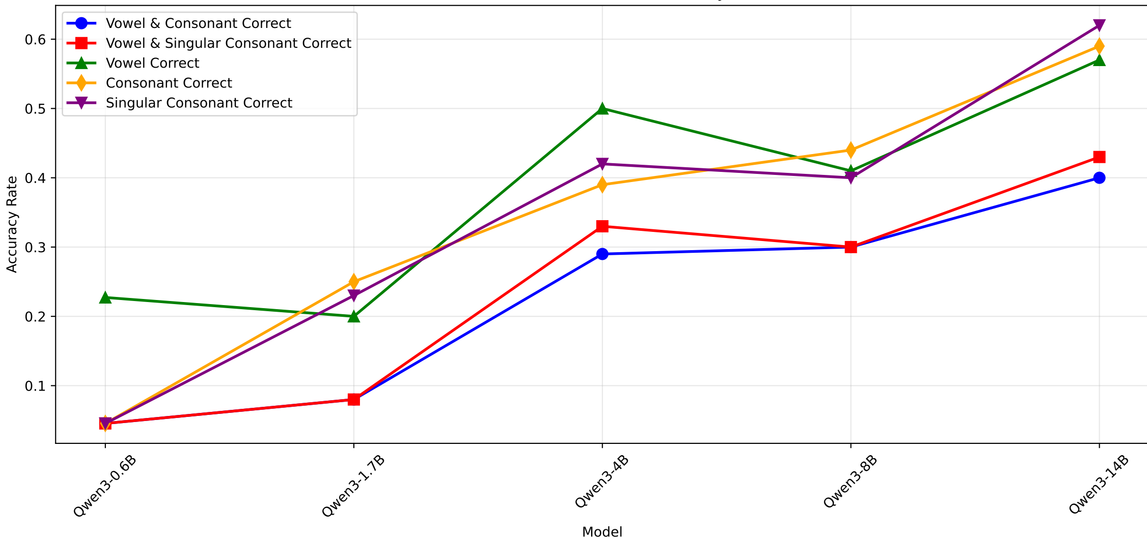
Vowel and Consonant Correctness by Model
