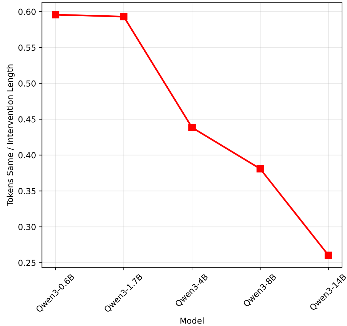
Tokens Same as % of Intervention Length
