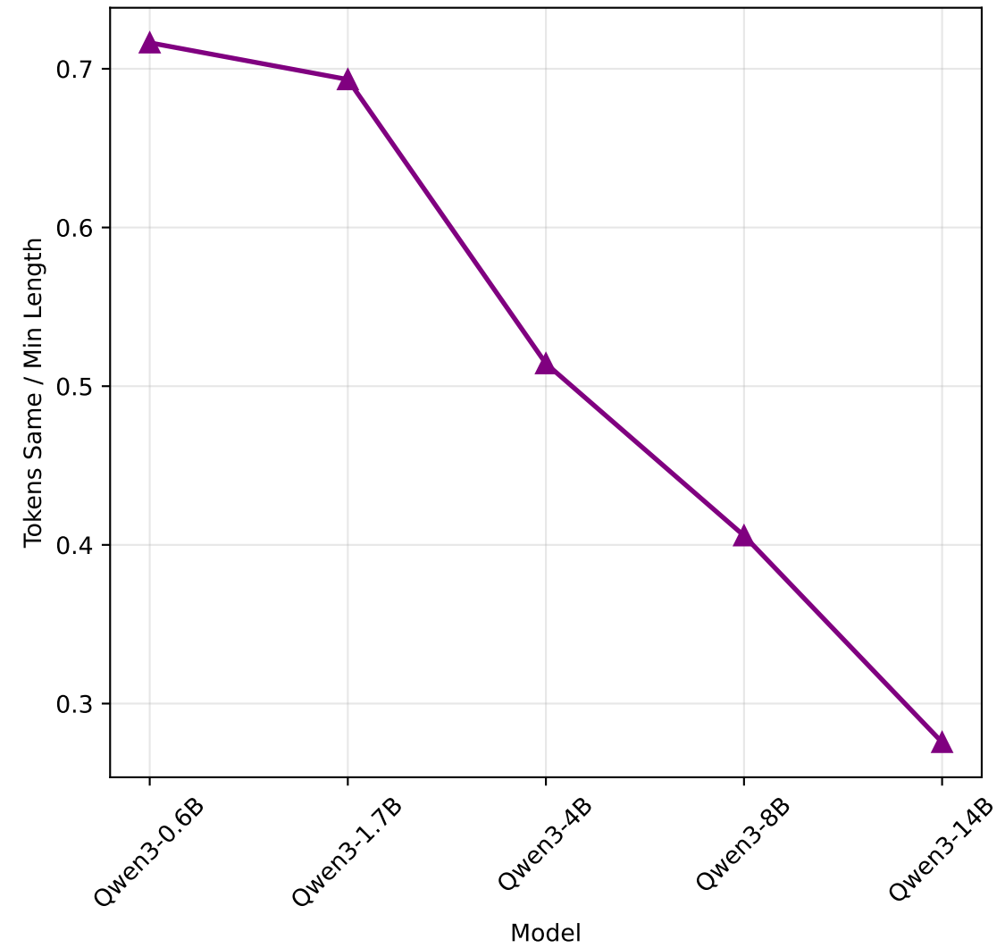
Tokens Same as % of Min Length
