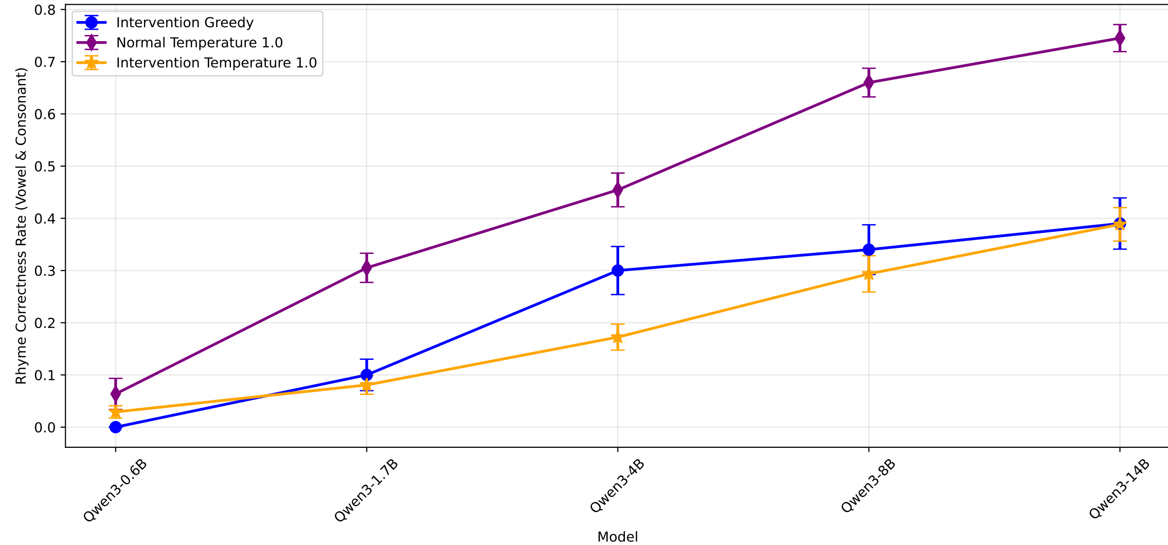
Rhyme Correctness by Model: Intervention vs Temperature 1.0 Sampling
