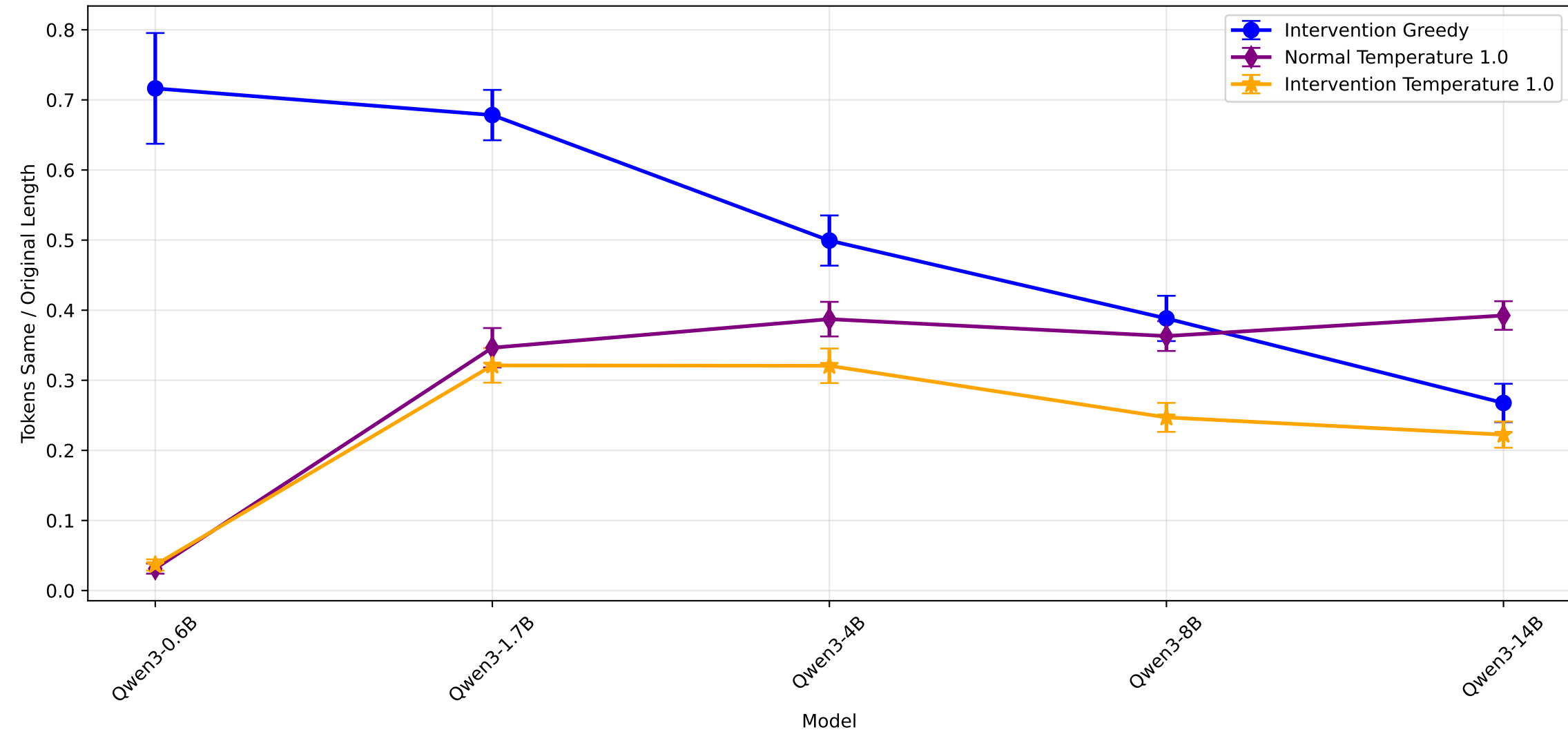
Tokens Same as % of Original Length: Intervention vs Temperature 1.0 Sampling
