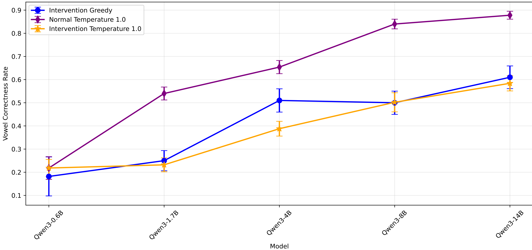
Vowel Correctness by Model: Intervention vs Temperature 1.0 Sampling
