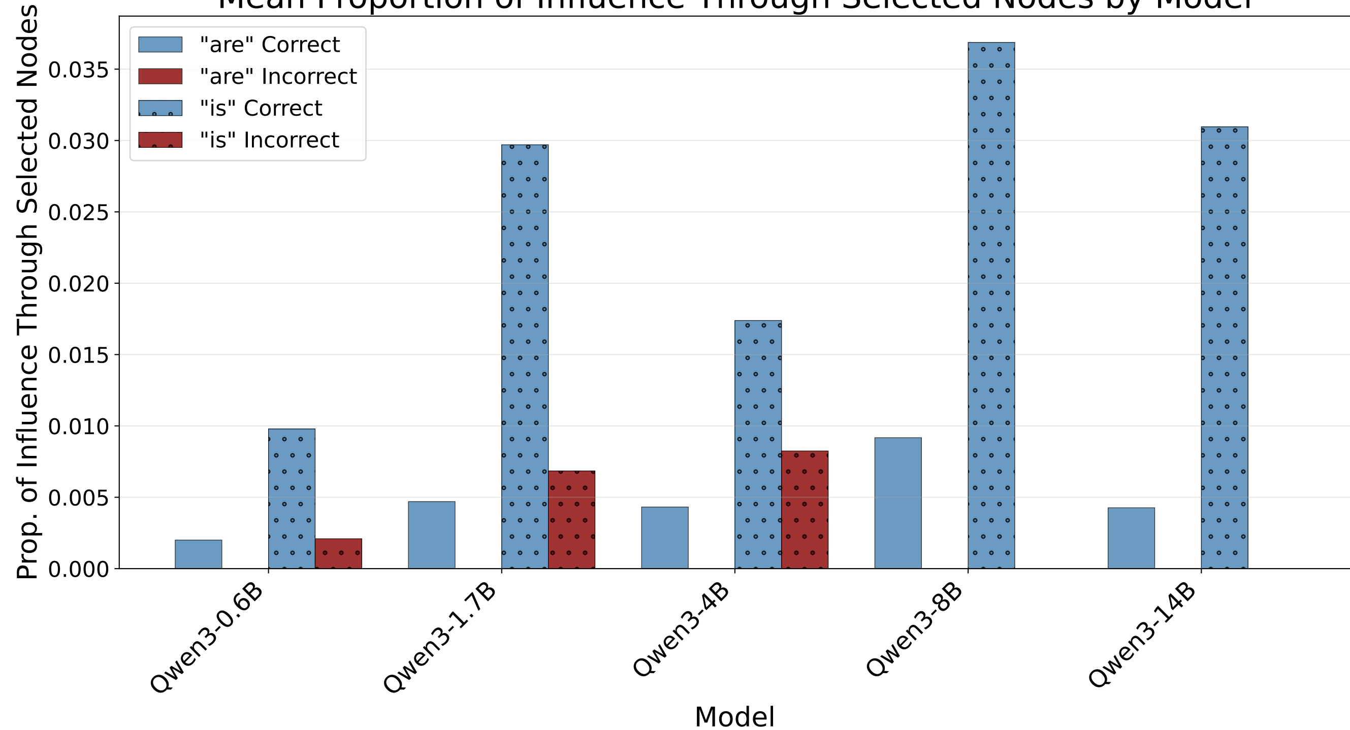
Mean Proportion of Influence Through Selected Nodes by Model
