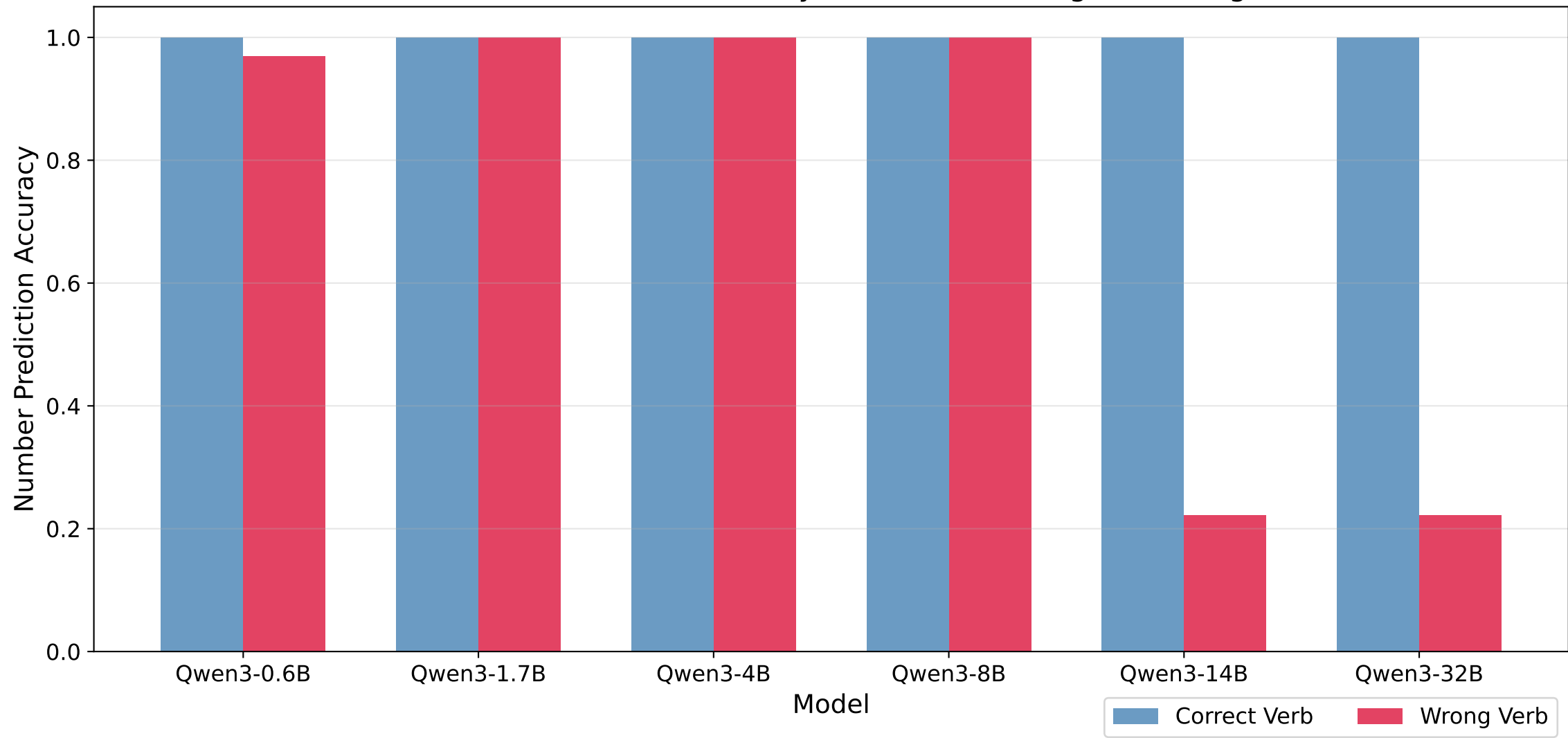
Number Prediction Accuracy: Correct vs Wrong Verb Usage
