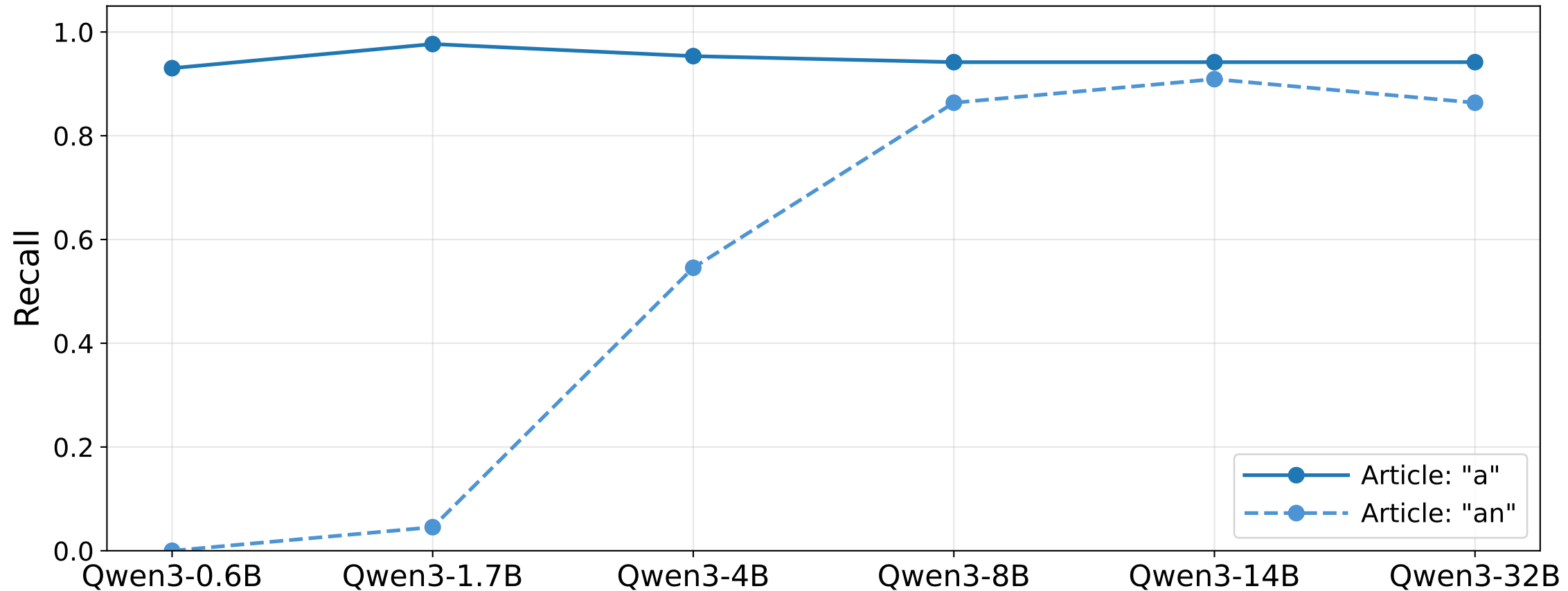
Article Recall Across Model Sizes (a/an)
