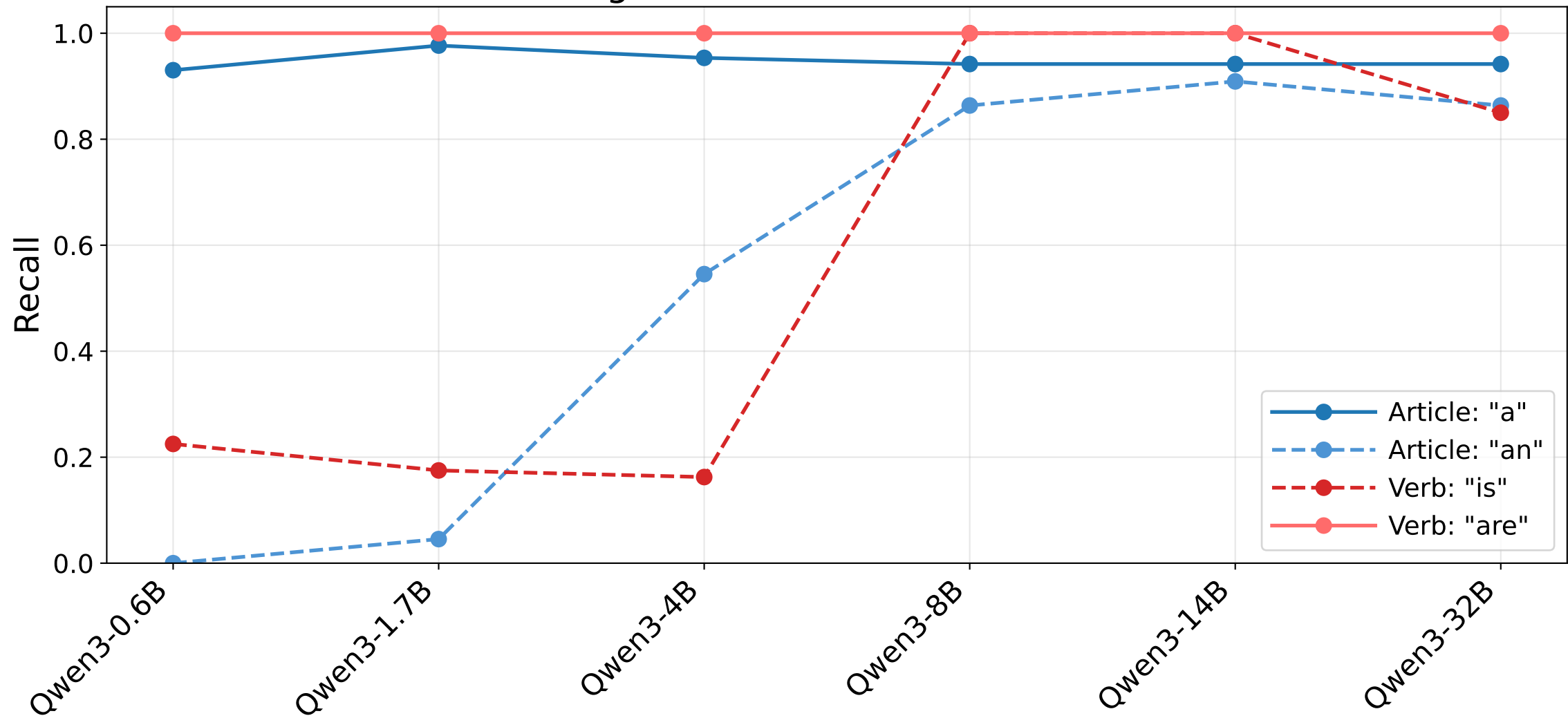
Planning Task Recall Across Model Sizes
