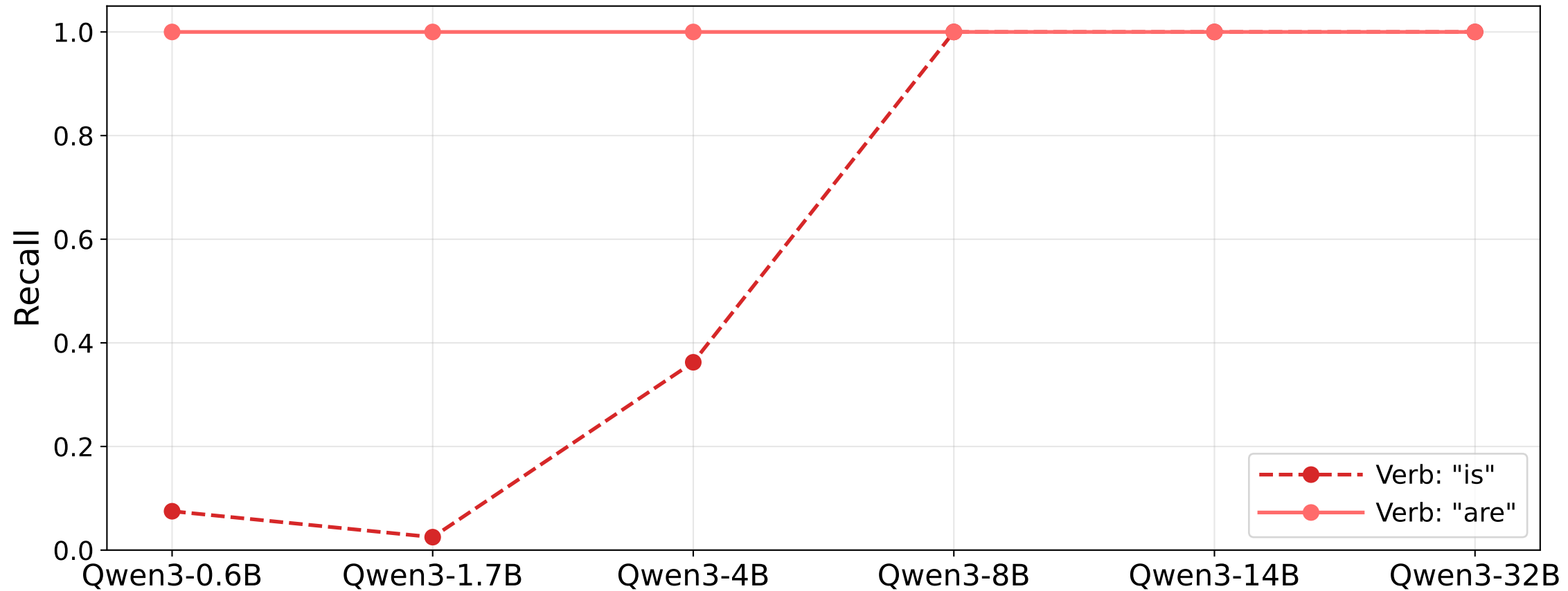
Verb Recall Across Model Sizes (is/are)
