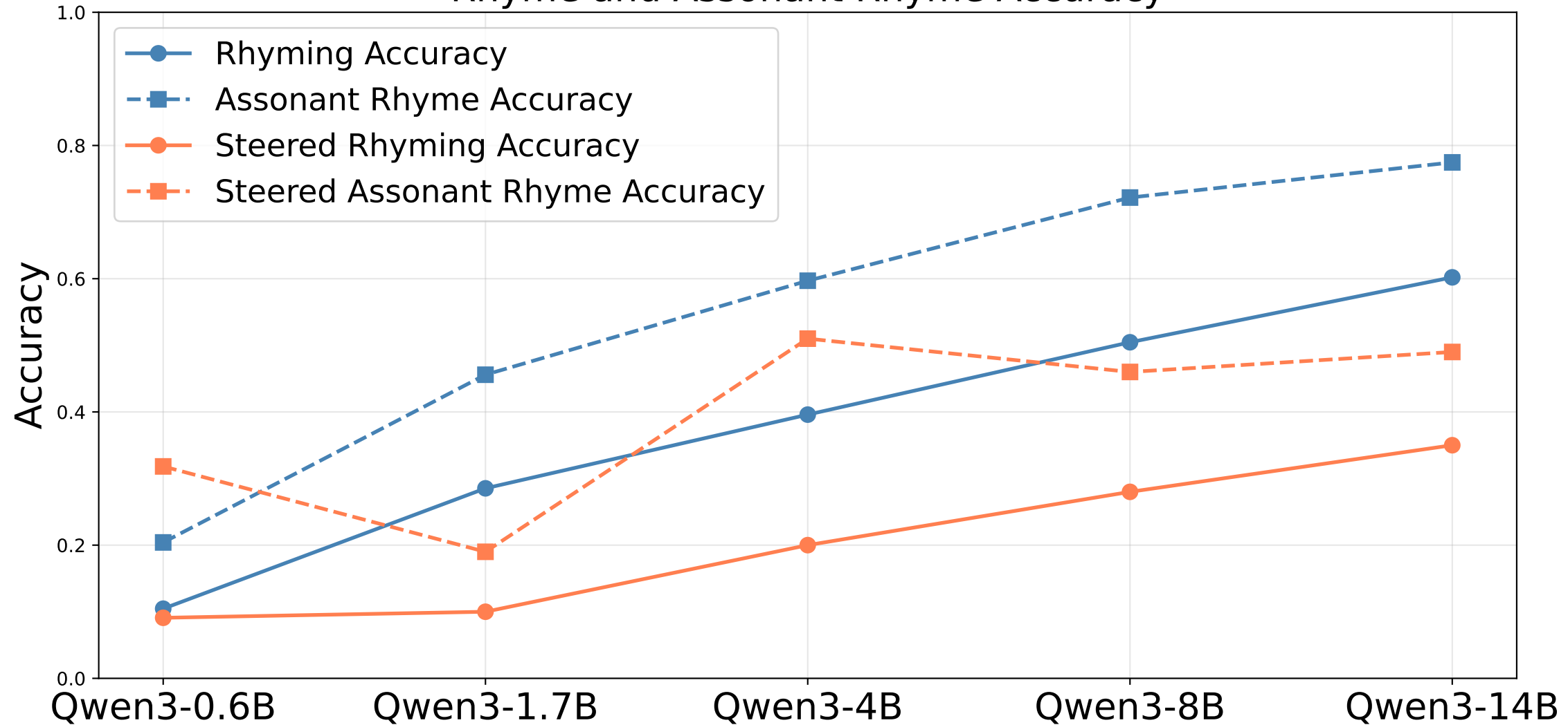
Rhyme and Assonant Rhyme Accuracy
