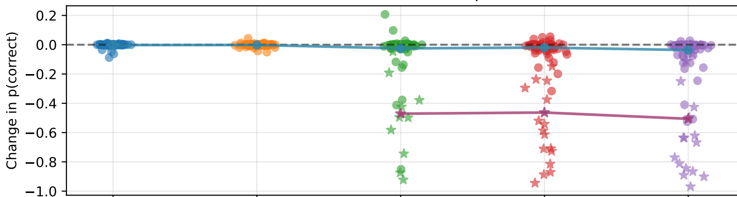
Normal Intervention Effect of Zero Ablations on p(\text{correct})
