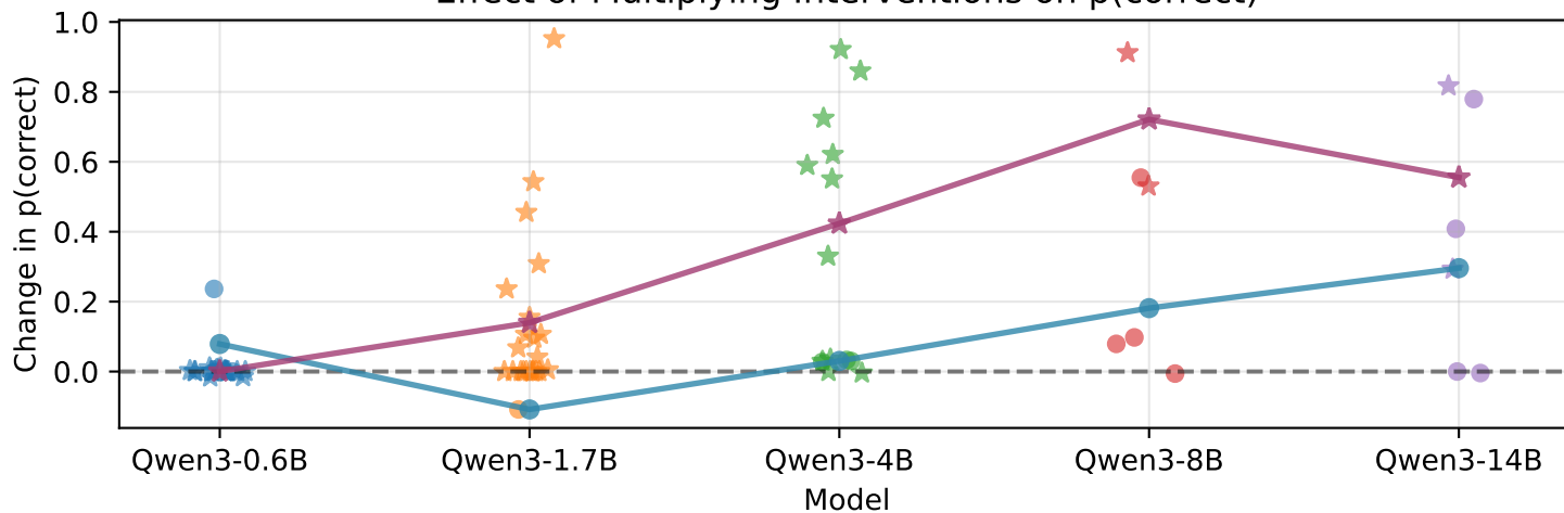
Effect of Multiplying Interventions on p(\text{correct})
