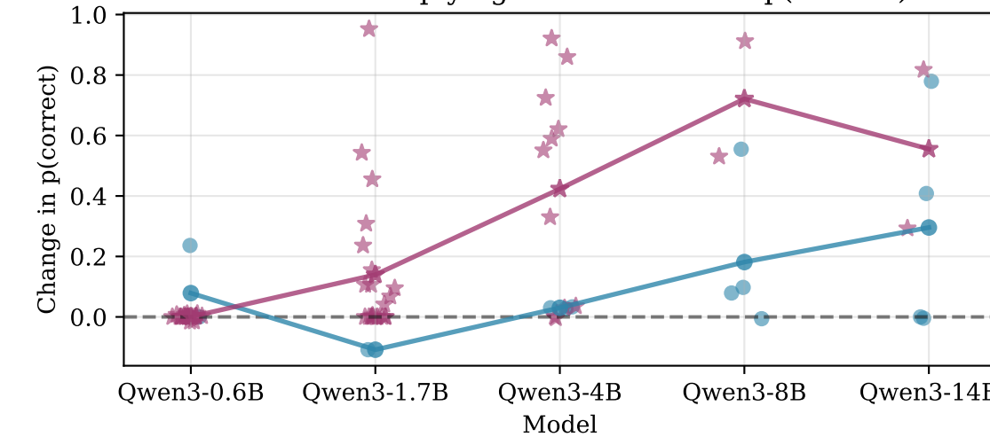
Effect of Multiplying Interventions on p(correct)
