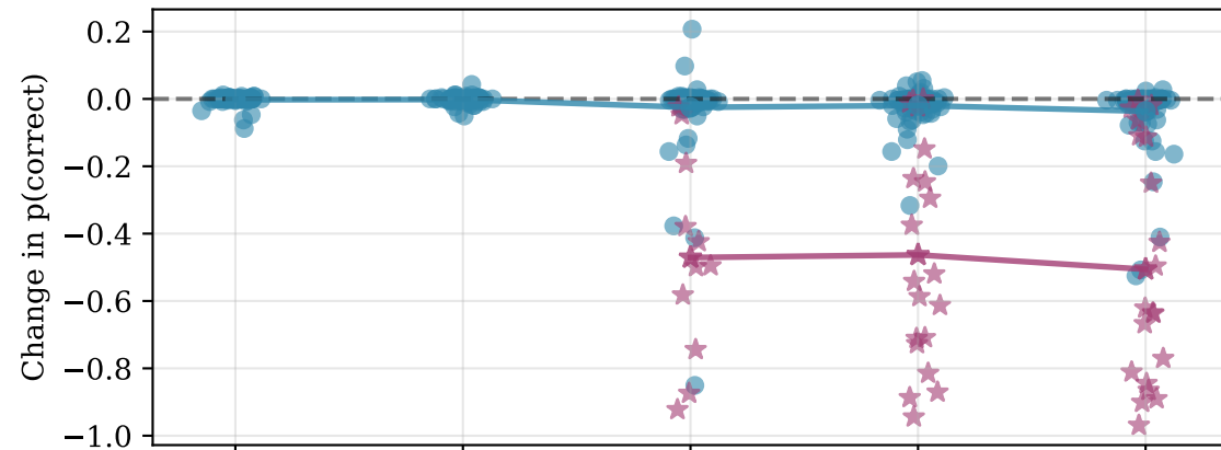
Effect of Multiplying Interventions on p(correct)
