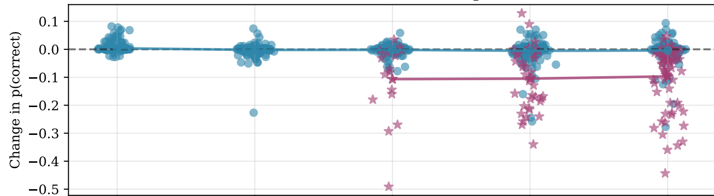
Direct Intervention Effect of Zero Ablations on p(correct)
