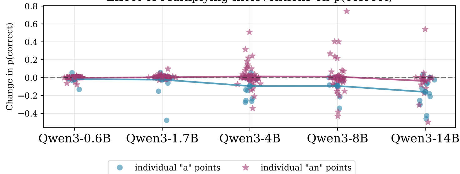
Effect of Multiplying Interventions on p(correct)
