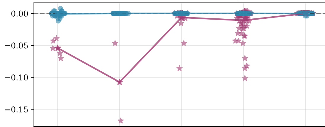
Effect of Direct Zero Ablations on p(correct)
