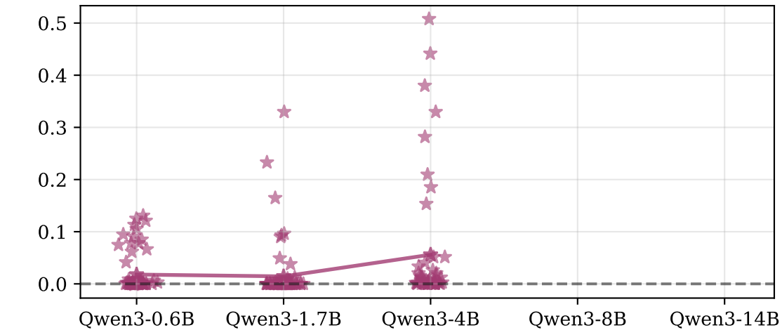
Effect of Direct Multiplying Interventions on p(correct)
