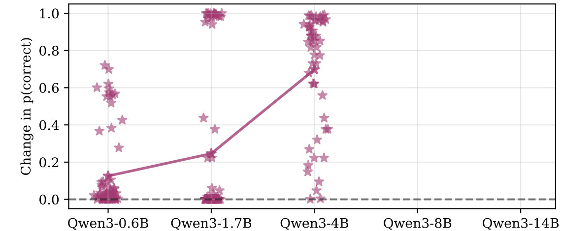
Effect of Multiplying Interventions on p(correct)
