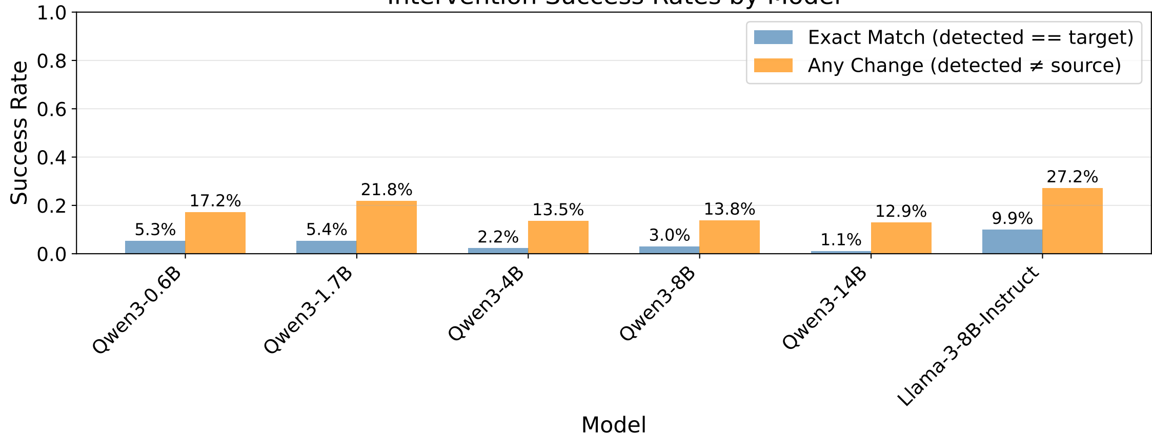
Intervention Success Rates by Model
