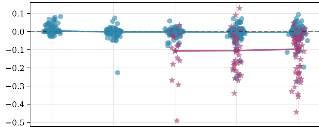
Effect of Direct Zero Ablations on p(correct)
