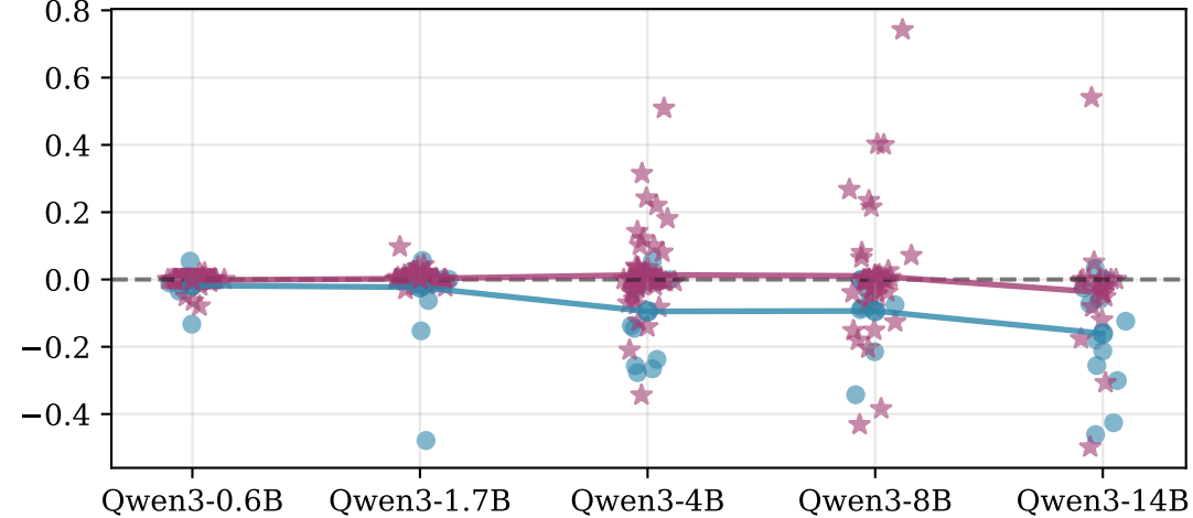
Effect of Direct Multiplying Interventions on p(correct)
