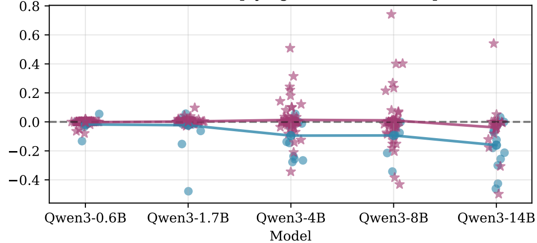
Effect of Direct Multiplying Interventions on p(correct)
