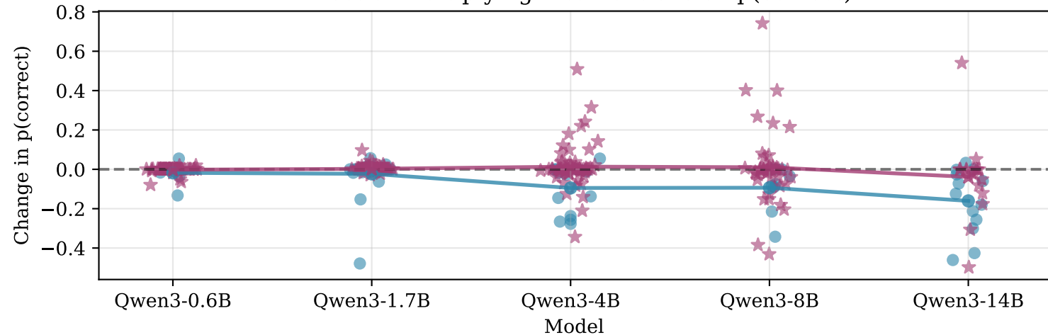
Effect of Multiplying Interventions on p(correct)
