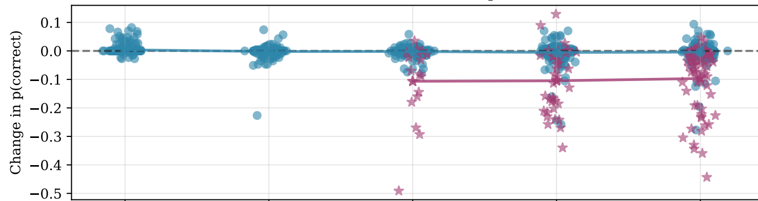
Direct Intervention Effect of Zero Ablations on p(correct)
