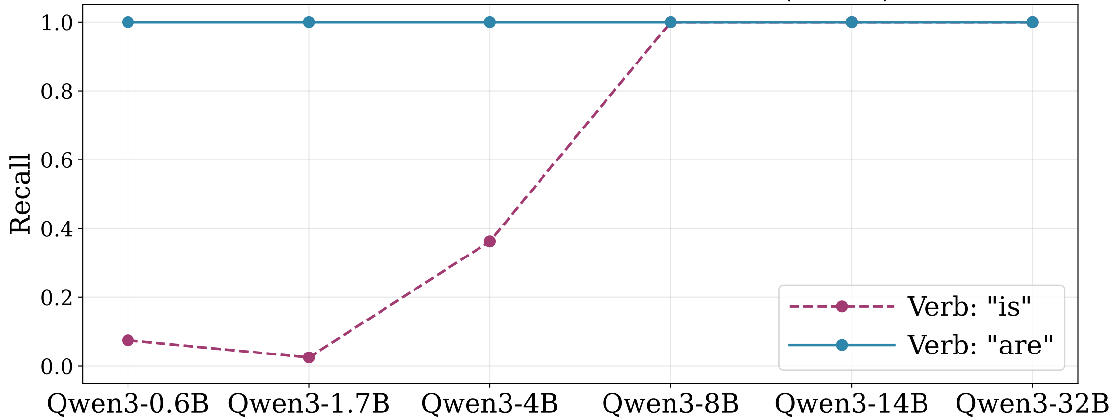
Verb Recall Across Model Sizes (is/are)
