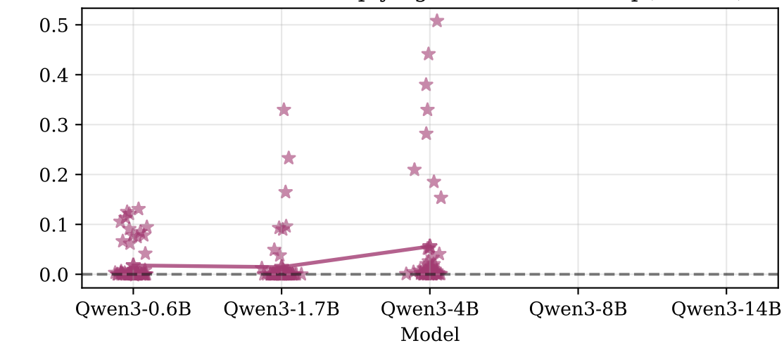
Effect of Direct Multiplying Interventions on p(correct)
