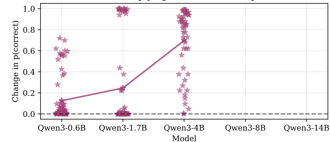
Effect of Multiplying Interventions on p(correct)
