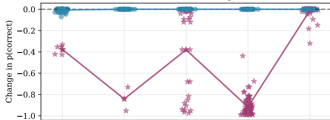
Effect of Zero Ablations on p(correct)
