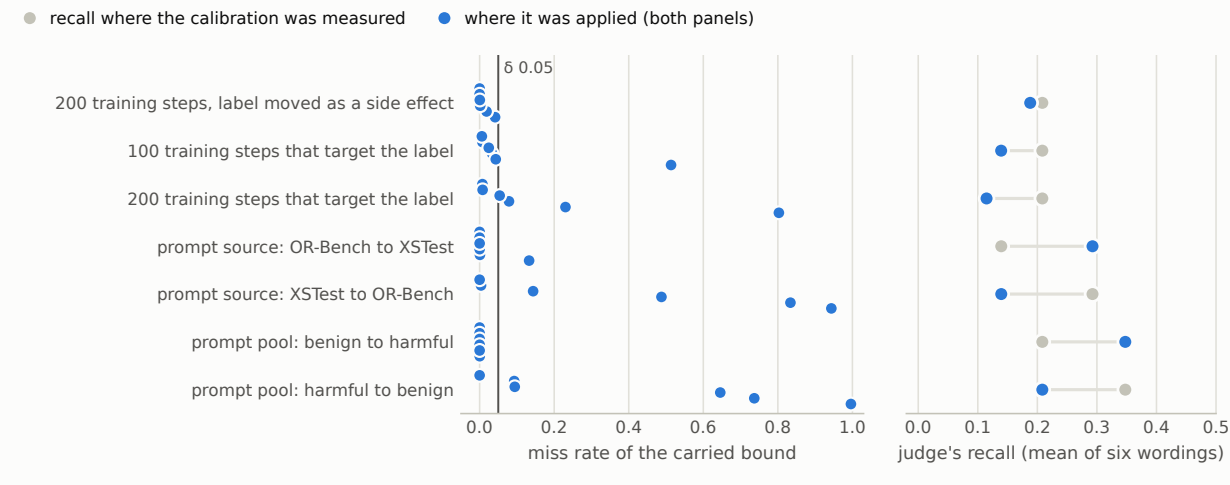
Figure 3. A carried calibration: miss rate of the carried bound and the judge’s recall, by shift.
