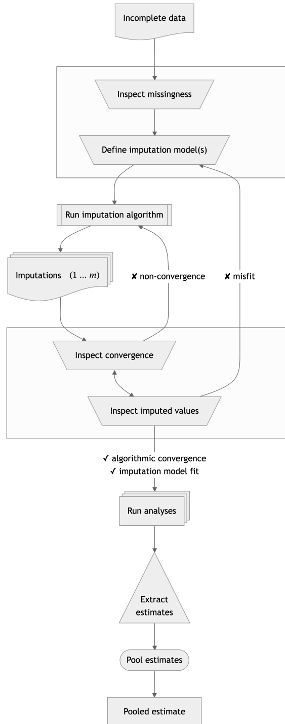
Figure 4: Multiple imputation flowchart
