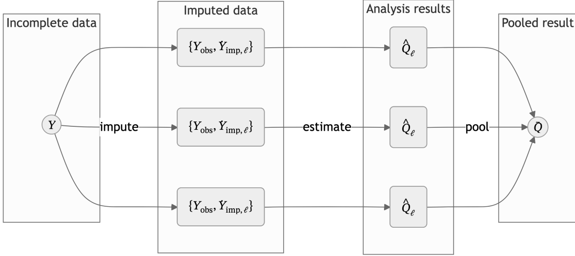
Figure 3: Multiple imputation scheme ( m = 3 )
