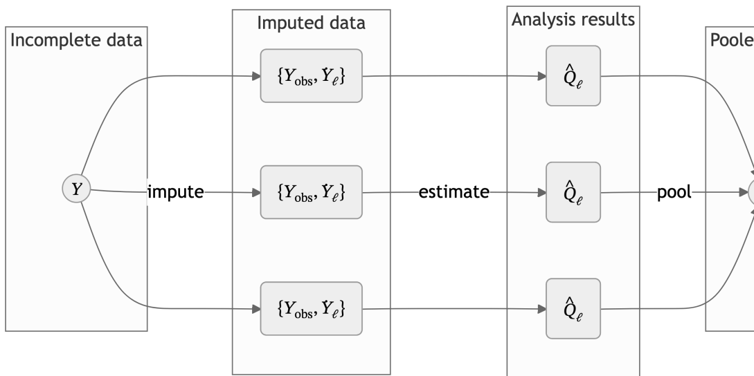
Figure 4: Multiple imputation scheme ( m = 3 )
