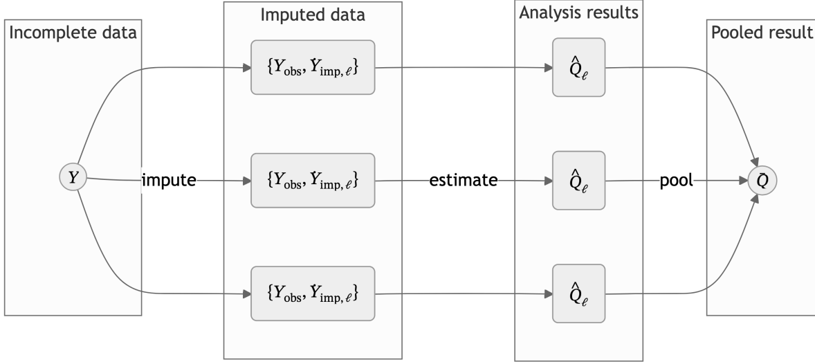
Figure 3: MI workflow
